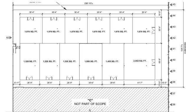
1 ENLARGED WAREHOUSE FLOOR PLAN SCALE: 1" = 20'-0"
